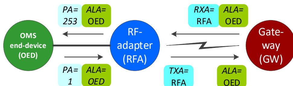
Figure 14 – Address usage in FFC with RF-Adapter
