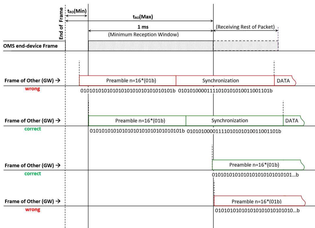
Figure 17 – Access timing of an OMS end-device with short access windows (Mode C2 example)
