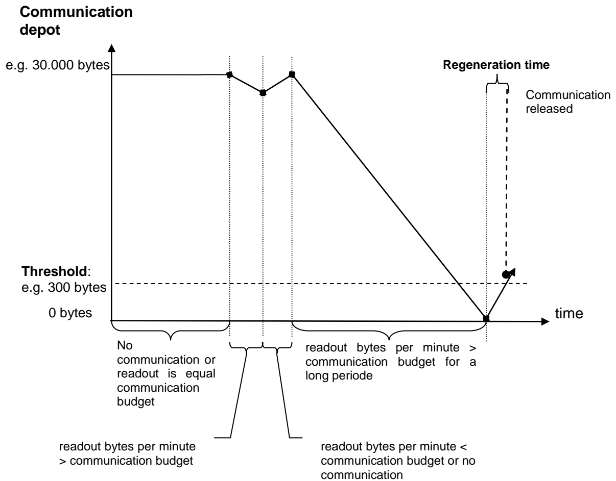
Figure P.8 - Communication depot
